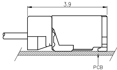
MATED CONDITION
